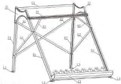
70MM Type Bracket
