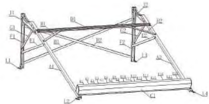
U Type Bracket
